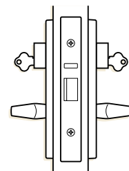
Non-Monitored Lock with Key Override Both Sides (Reversible) 3574ELN2 Series
